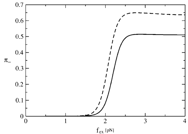
FIGURE 11 The fraction of backward steps, \pi_- , is insignificant in the model until an external force of \sim 2 \text{ pN} is reached. The solid line is for [ATP] = 2 \text{ mM} and [ADP] = 200 \mu\text{M} , while the dashed line is for a reduced ATP concentration of 100 \mu\text{M} .
