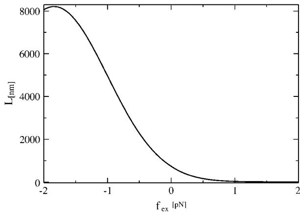
FIGURE 10 Run length L for different strengths of the external force when [ATP] = 1 \text{ mM} and [ADP] = 200 \mu\text{M} . For negative external force, the run length has a nonmonotonic behavior, where it increases 10-fold before decreasing again.
