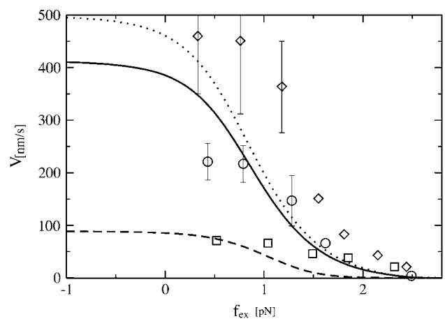
FIGURE 6 The velocity as a function of force. The solid line (and circles) show results when [ATP] = 1 \text{ mM} and [ADP] = 200 \mu\text{M} , the dashed line (and squares) when [ATP] = 1 \text{ mM} and [ADP] = 1 \mu\text{M} , while for the dotted line (and diamonds) we have [ATP] = 10 \mu\text{M} and [ADP] = 1 \mu\text{M} . The model (the lines) shows similar trends to what is found experimentally (the circles, squares, and diamonds) (25).
