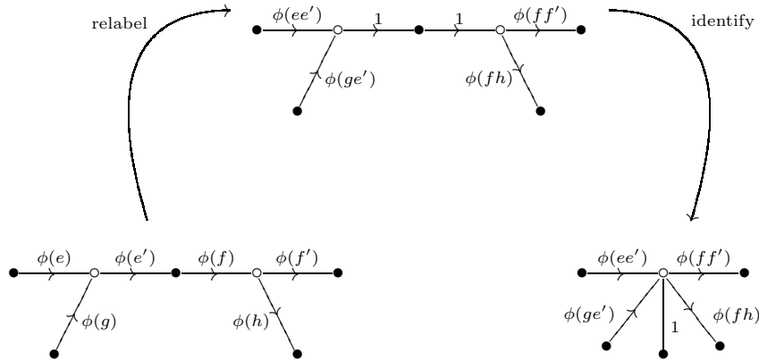
FIGURE 3. Relabellings and identifications in case 1.
