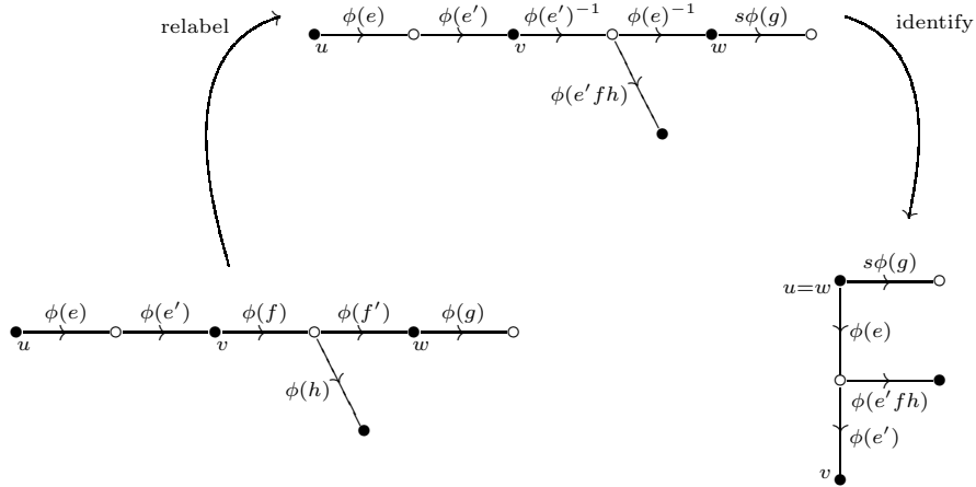
FIGURE 4. Relabellings and identifications in case 2.
