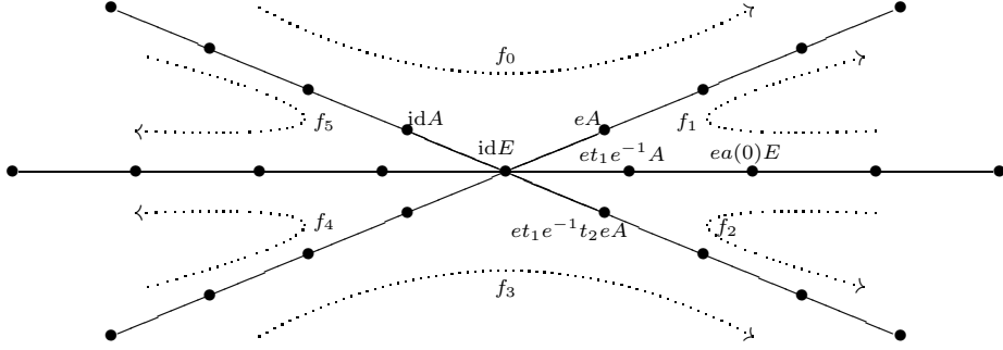
FIGURE 7. A 6-pod with all branches of length 4 (example 46)
