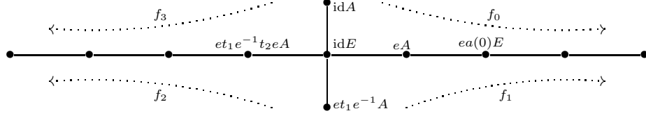
FIGURE 8. A 4-pod with branches 4,1,4,1 (example 47)
