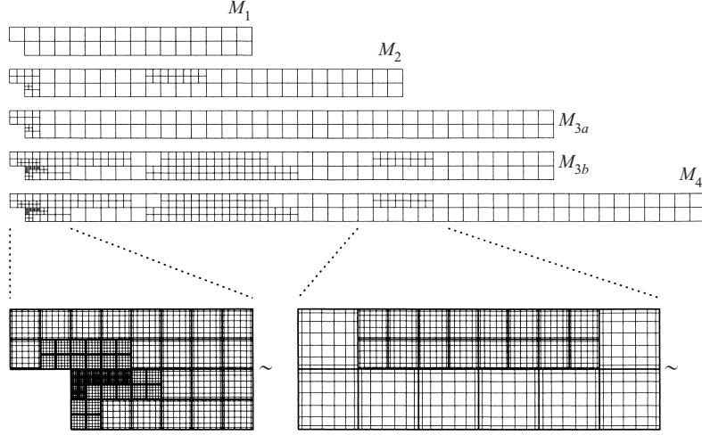
FIGURE 2. Computational domains used in the present study. Subscripts label external dimensions (specifically outflow length L_o ). Each domain is divided into K elements. Where necessary, lower-case letters label the degree of internal mesh refinement: the M_{3a} mesh has K = 83 elements and the M_{3b} mesh has K = 203 elements. Within each element the solution and geometry are represented by N^2 polynomial coefficients. Two subsections of mesh M_4 are expanded to show the internal distribution of quadrature points for polynomial order N = 7 . To simulate a three-dimensional flow the solution is decomposed into M Fourier modes in the periodic spanwise direction, each computed on the same two-dimensional grid.
