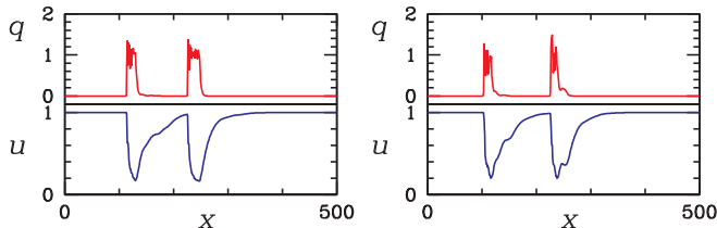
FIG. 9. (Color online) Further effect of parameter \beta . (Left) \beta = 0.3 ( R = 1980 ); (right) \beta = 0.5 ( R = 2180 ). In each case snapshots of solutions are shown just after a puff split. There is little to distinguish the cases.
