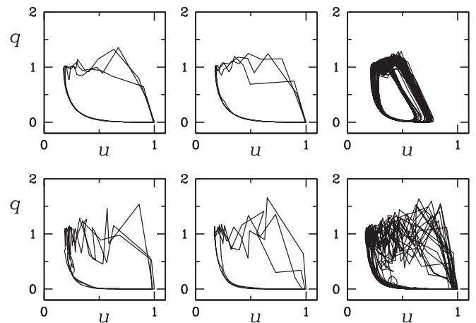
FIG. 7. Effect of parameter k . Top row, k = 1 ; bottom row, k = 2 . In each case snapshots are plotted in the u - q phase plane. The left two plots show randomly chosen snapshots of solutions with three closely spaced puffs. The rightmost plots are of solutions following a quench from high R and contain a large number of puffs. Top row is at R = 1760 and the bottom row is at R = 2000 . Both values of R are close to the transition to sustained turbulence for the corresponding value of k .
