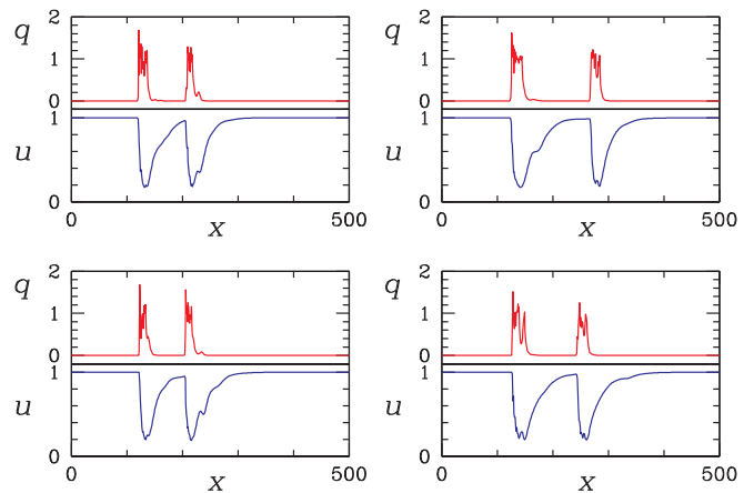
FIG. 11. (Color online) Effect of parameters c and d . In each case snapshots of solutions are shown just after puff splitting. Splitting is not very sensitive to c and d around values used in the paper. (Top left) c = 0.45 , d = 0.1 , R = 2480 ; (top right) c = 0.45 , d = 0.2025 , R = 1960 ; (bottom left) c = 0.35 , d = 0.15 , R = 2120 ; (bottom right) c = 0.55 , d = 0.15 , R = 2080 .
