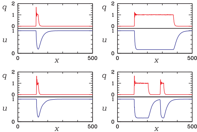
FIG. 8. (Color online) Effect of parameter \beta . Top row, \beta = -0.4 ; bottom row, \beta = 0 . In each case snapshots of solutions are shown on either side on the transition from localized puffs to expanding turbulence. (Top left) R = 1750 ; (top right) R = 1780 ; (bottom left) R = 1760 ; (bottom right) R = 1800 .
