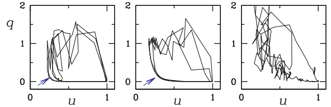
FIG. 10. (Color online) Effect of parameter \gamma . (Left) \gamma = 0.80 , with R = 2400 ; (middle) \gamma = 0.95 , with R = 2000 , and is the same plot as bottom middle of Fig. 7. Arrows indicate the relevant region of the u - q phase plane. (Right) DNS of a puff at Re = 2000 , exactly the same as in Fig. 6.
