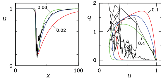
FIG. 6. (Color online) Parameters \epsilon_1 and \epsilon_2 chosen to match a typical puff from DNS at Re = 2000 . In the left plot \epsilon_2 = 0.2 , while \epsilon_1 has values 0.02 (red), 0.04 (blue), and 0.06 (green). In the right plot \epsilon_1 = 0.04 and \epsilon_2 has values 0.1 (red), 0.2 (blue), and 0.4 (green). r = 0.7 . DNS is the irregular black curve. The unlabeled (blue) curves in the two plots correspond to the values of \epsilon_1 and \epsilon_2 used in the paper.
