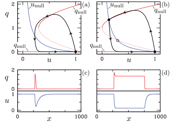
FIG. 2. (Color online) The distinction between puffs and slugs seen as the difference between excitability and bistability in Eqs. (1) and (2). Phase planes show nullclines at (a) r = 0.7 and (b) r = 1 . The fixed point (1,0) corresponds to parabolic flow. In (b) the additional stable fixed point corresponds to stable turbulence. Solution snapshots show (c) a puff at r = 0.7 and (d) a slug at r = 1 . These solutions are plotted in the phase planes with arrows indicating increasing x .
