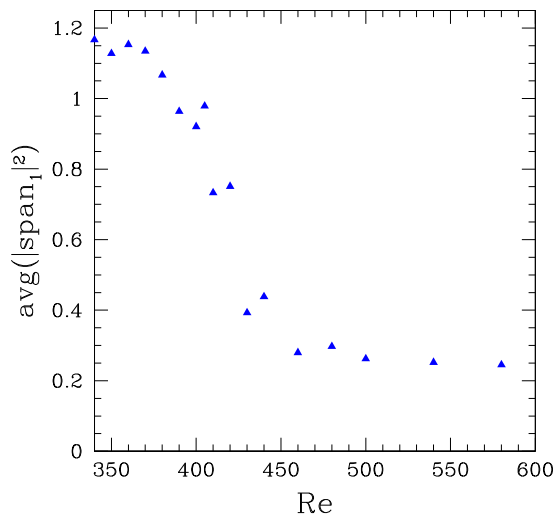
FIG. 6. (Color online) Square modulus of Fourier component corresponding to pattern wavelength as a function of Reynolds number.
