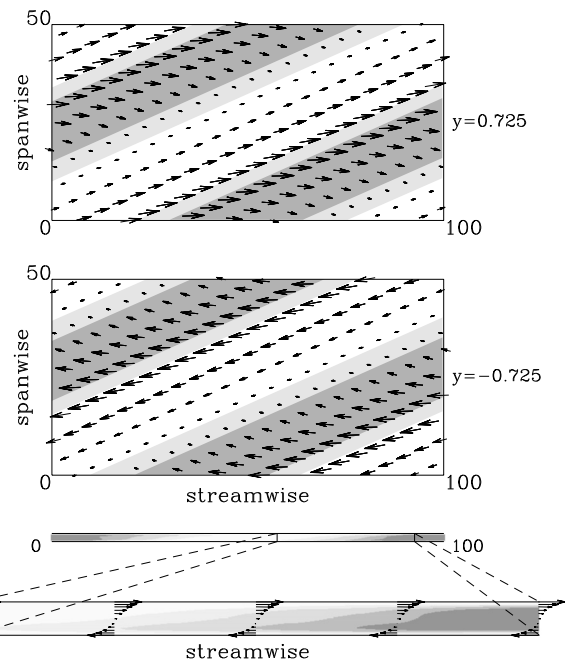
FIG. 14. Mean velocity components seen in three planes with standard orientation for Couette flow. The turbulent regions are shaded. Top: velocity components in the streamwise-spanwise plane at y=0.725 (upper part of the channel). Middle: same except y=-0.725 (lower part of the channel). Bottom: flow in a constant spanwise cut. The mean velocity is shown in the enlarged region.
