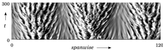
FIG. 2. Streamwise velocity along a line oriented in the spanwise direction in the midplane at Re=350 . Streaks move out from the center of the turbulent region toward the laminar regions. The flow is the same as that in Fig. 1.
