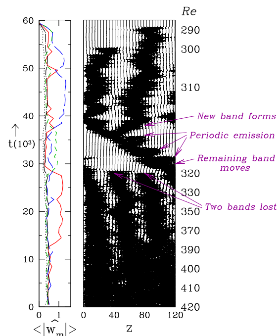
FIG. 4. (Color online) As in Fig. 3, but with slightly different Reynolds number history. Two turbulent bands disappear at Re=320 , leading to translation of the single remaining band with the eventual reappearance of a stationary pattern with two bands.
