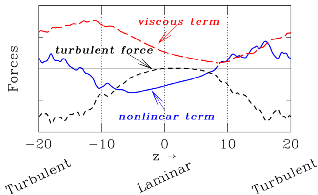
FIG. 15. (Color online) Mean forces in x direction as a function of z at y=0.725 for turbulent-laminar pattern at Re=350 . Advective -(\mathbf{U} \cdot \nabla)U (blue, solid), viscous \nabla^2 U/Re (red, dashed), and turbulent -\langle(\tilde{\mathbf{u}} \cdot \nabla)\tilde{\mathbf{u}}\rangle (black, short-dashed) forces. In the laminar region ( z \approx 0 ), the Reynolds-stress force vanishes and the viscous and advective forces are equal and opposite to one another.
