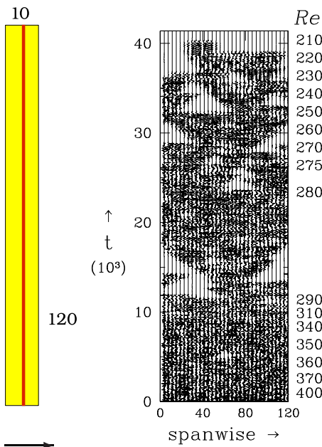
FIG. 11. (Color online) Evolution in a domain with streamwise extent L_x = 10 and spanwise extent L_z = 120 . Timeseries taken at points along long spanwise direction indicated by red line. Turbulent regions subsist far below Re = 300 .
