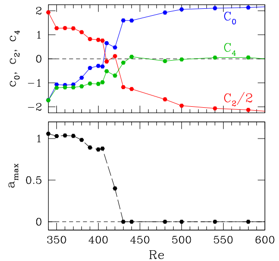
FIG. 8. (Color online) Top: fitting coefficients for quartic functional form (6). Quartic coefficient c_4 becomes negligible for Re \geq 430 , coefficients c_0 , c_2 change sign near this value as well. Bottom: most probable value of a is zero for Re \geq 430 .
