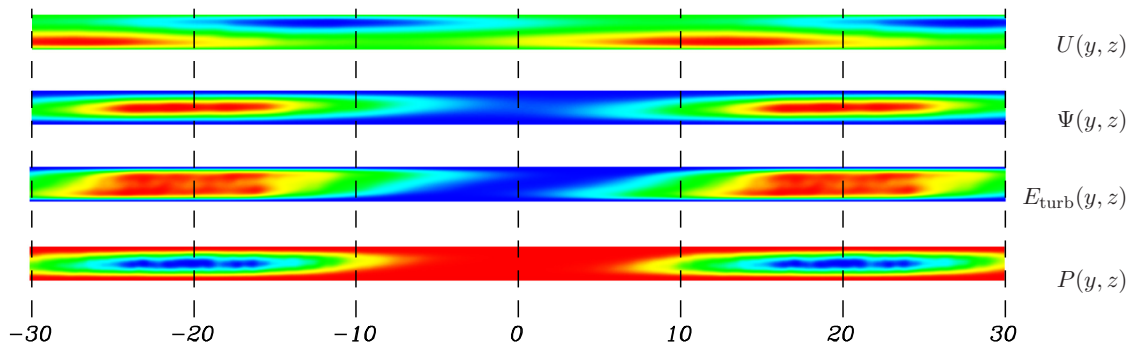
FIG. 13. (Color online) U(y, z) : transverse component of mean flow. \Psi(y, z) : streamfunction of in-plane mean flow. A long cell extends from one laminar-turbulent boundary to the other. Gradients of \Psi are much larger in y than in z , i.e., |W| \gg |V| . In the laminar region at the center, W, V \approx 0 . E_{\text{turb}}(y, z) : mean turbulent kinetic energy \langle \tilde{\mathbf{u}} \cdot \tilde{\mathbf{u}} \rangle / 2 . There is a phase difference of \lambda_z/4 = 10 between extrema of E_{\text{turb}} and U . P(y, z) : mean pressure field. Pressure gradients are primarily in the y direction and within the turbulent region. Color ranges for each field from blue to red: U [-0.4, 0.4] , \Psi [0, 0.09] , E_{\text{turb}} [0, 0.4] , P [0, 0.007] .
