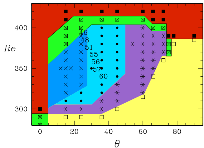
FIG. 9. (Color online) Survey of turbulent-laminar patterned regimes in our computations of plane Couette flow as a function of imposed angle \theta and Reynolds number Re . Uniform turbulence (solid squares, red), intermittent (green, crosses in squares), turbulent-laminar patterns with wavelength of 40 (blue, crosses) or 60 (light blue, dots), localized states (stars, purple), laminar Couette flow (hollow squares, yellow). Numbers show wavelengths found in experiments (Ref. 3) at appropriate values of \theta and Re .
