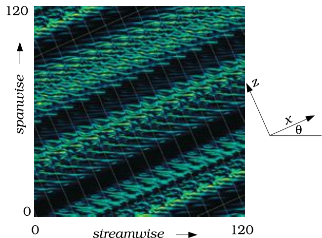
FIG. 1. (Color online) Computed turbulent-laminar pattern at Re=350 . Shown is the kinetic energy at y=0 , midway between bounding plates at y=\pm 1 which move to the right and left in the streamwise direction. Turbulent bands consist of streamwise streaks and vortices. The bands are oriented in the direction denoted by x at an angle of 24^\circ from the streamwise direction, and are separated by a wavelength of 40 in the direction of the pattern wavevector, denoted by z .
