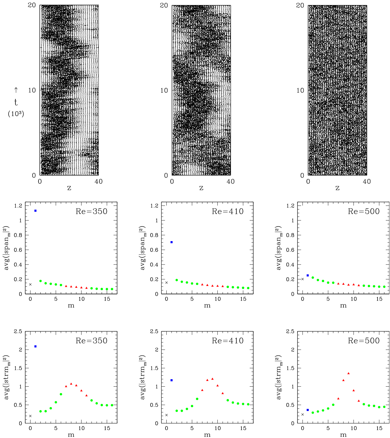
FIG. 5. (Color online) Left column: statistically steady turbulent-laminar pattern at Re=350 . Middle column: intermittent state at Re=410 . Right column: uniform turbulence at Re=500 . Top row: timeseries of the spanwise velocity along the line x=y=0 at 32 equally spaced values of z . Middle row: time-average of the power spectrum in z of the spanwise velocity. Bottom row: time-average of the power spectrum of the streamwise velocity. The blue square at m=1 corresponds to the pattern wavelength of 40. The red triangles at 7 \leq m \leq 11 correspond to streamwise streaks. The m=0 component is shown as a black cross and the remaining components are shown as green dots.
