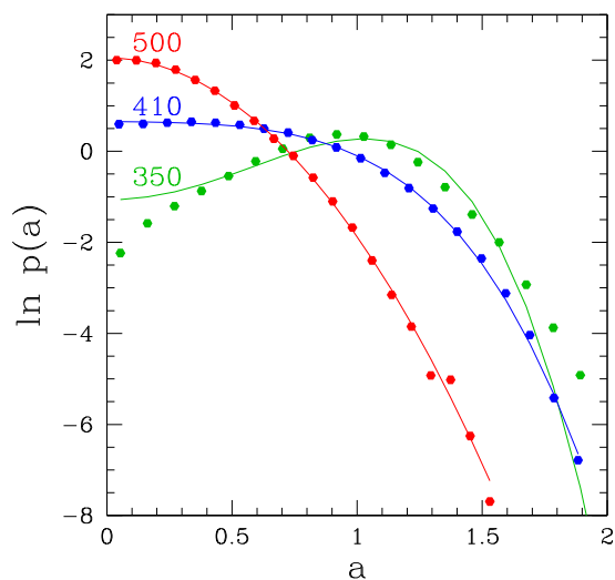
FIG. 7. (Color online) Logarithm \ln p(a) for the modulus a of the first Fourier component, for a uniformly turbulent flow at Re=500 , an intermittent flow at Re=410 , and a turbulent-laminar patterned flow at Re=350 . The most probable value is a=0 for uniform turbulence but has a finite value for a patterned flow. Points are obtained by Fourier transforming and binning the data in Fig. 5. Curves are fits to quartic functions.
