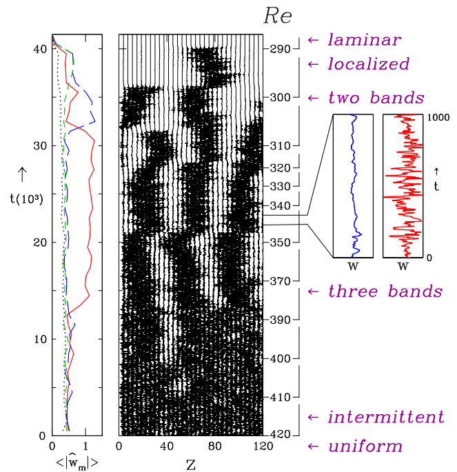
FIG. 3. (Color online) Timeseries in domain with L_z=120 . Middle: spanwise velocity at 32 points along a line in the midplane x=y=0 as the Reynolds number is decreased. Left: modulus of Fourier transform in the z direction, averaged over time windows of length \Delta T=1000 , showing evolution of components corresponding to wavelengths of 40 (solid red), 60 (long-dashed blue), 120 (short-dashed green), and \infty (dotted black). Right: evolution of spanwise velocity within laminar (left) and turbulent (right) bands over interval of length \Delta T=1000 . Transition to an intermittent regime is seen at Re=410 , to three bands at Re=390 , to two bands at Re=310 , to a localized state at Re=300 , and to laminar Couette flow at Re=290 .
