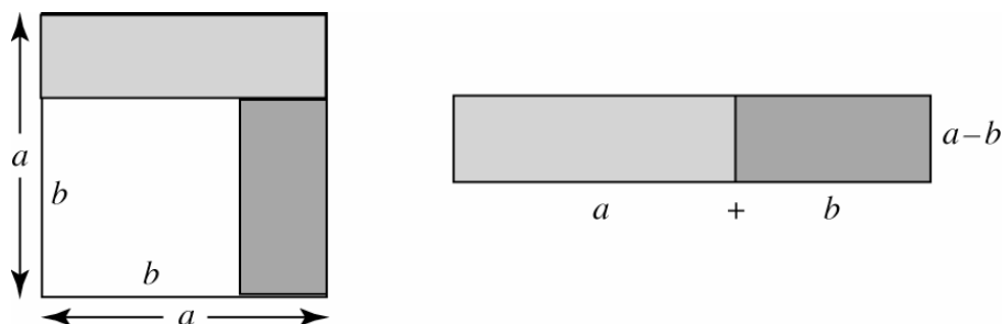
Figure 2: Take a square side b from a square side a and rearranging as (a-b) \times (a+b) .
