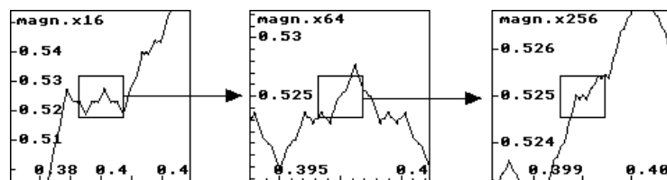
Figure 8: Successive magnifications show wrinkles at each level
