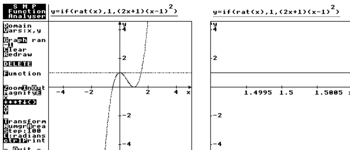
Figure 13 : The graph of y = \text{if}(\text{rat}(x), 1, (2x+1)(x-1)^2) , drawn to equal scales, then stretched horizontally to pull flat at x=1.5
