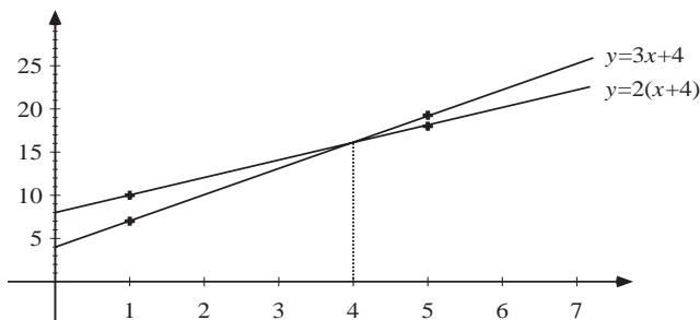
Figure 10 : Solving an equation graphically
