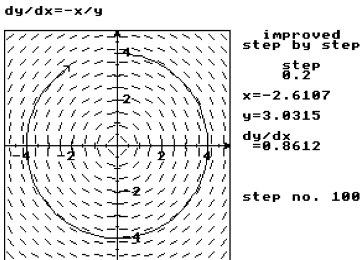
figure 4 : drawing a numerical solution of a first order differential equation
