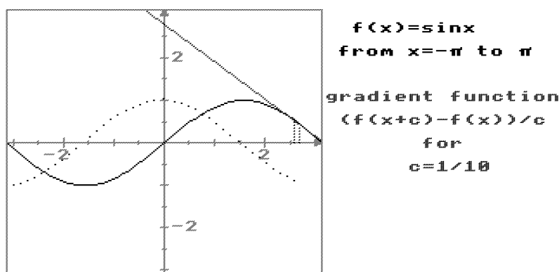
figure 2 : building up the gradient function of a graph
