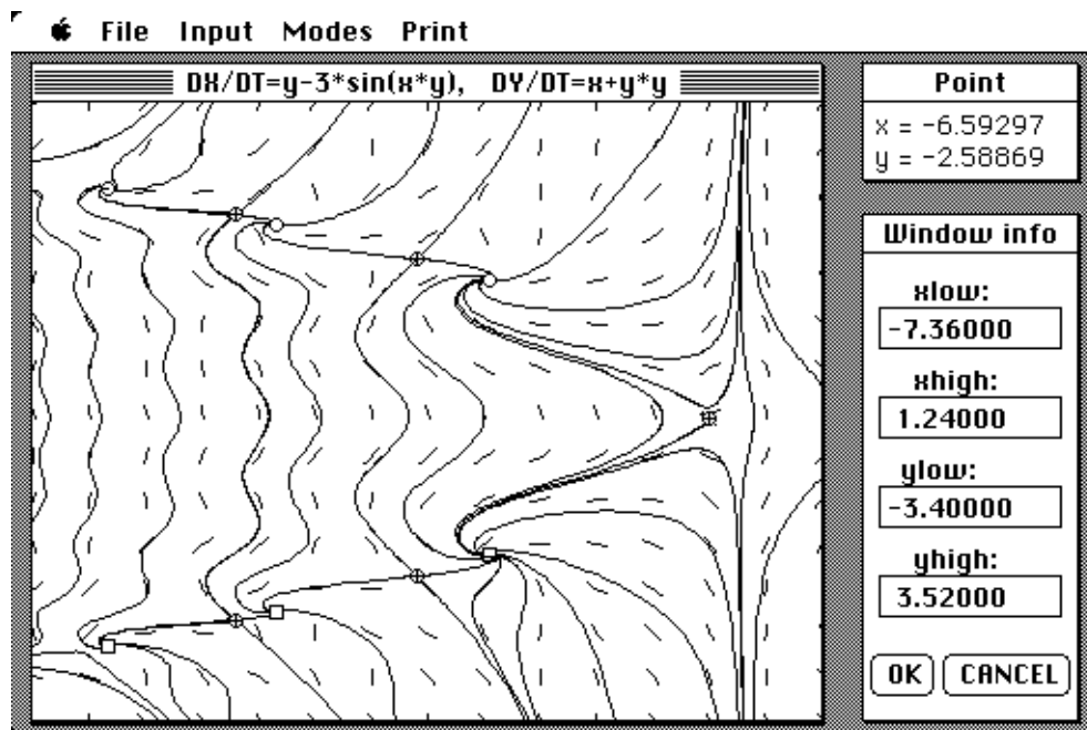
figure 8 : locating singular points and separatrices for saddle points
