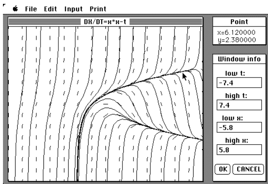
figure 5 : a family of solutions of a differential equation, showing funnel and antifunnel behaviour
