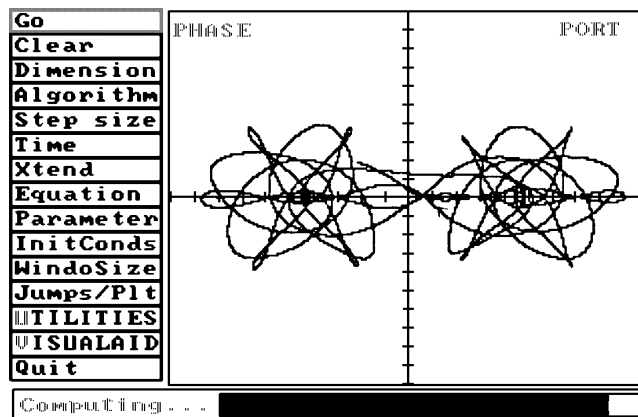
figure 7 : a numerical plot representing a tiny satellite orbiting two larger bodies
