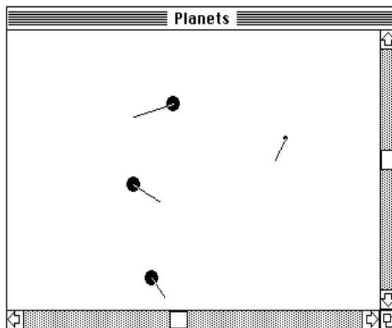
figure 6 : a numerical approximation to the many-body problem
