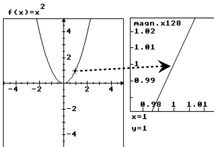
figure 1 : magnifying a small part of a graph to show its local straightness
