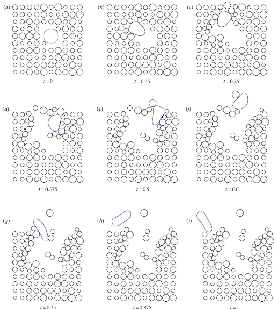
Figure 8. Undirected migration in the presence of obstacles of a cell under a combination of conserved surface tension and elastic evolution; for parameter values see table 1 and text. (Online version in colour.)
