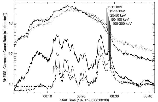
Fig. 1. A typical hard X-ray (25-300 keV) solar flare with quasi-periodic pulsations, observed in full disk measurements by RHESSI on the 19th of January, 2005. The event is associated with a flare of class X1.3 (peaking at 08:22 UT, as seen by GOES 1-8 Å).
