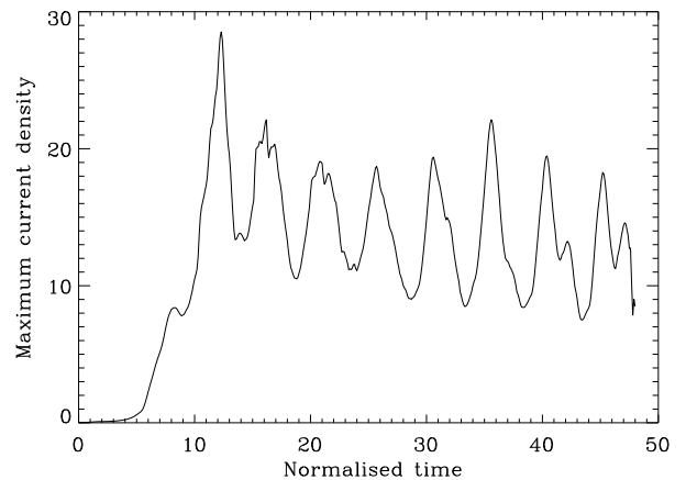
Fig. 3. Time evolution of the maximum electric current density in the vicinity of a 2D magnetic neutral point. The current is generated by a harmonic fast magnetoacoustic wave with the period 5 time units, coming towards the neutral point. The initial relative amplitude of the wave is 1.5%. The plasma \beta is finite. The normalising values are the magnetic field strength and the Alfvén speed at domain boundary, and the characteristic spatial scale of the field inhomogeneity.
