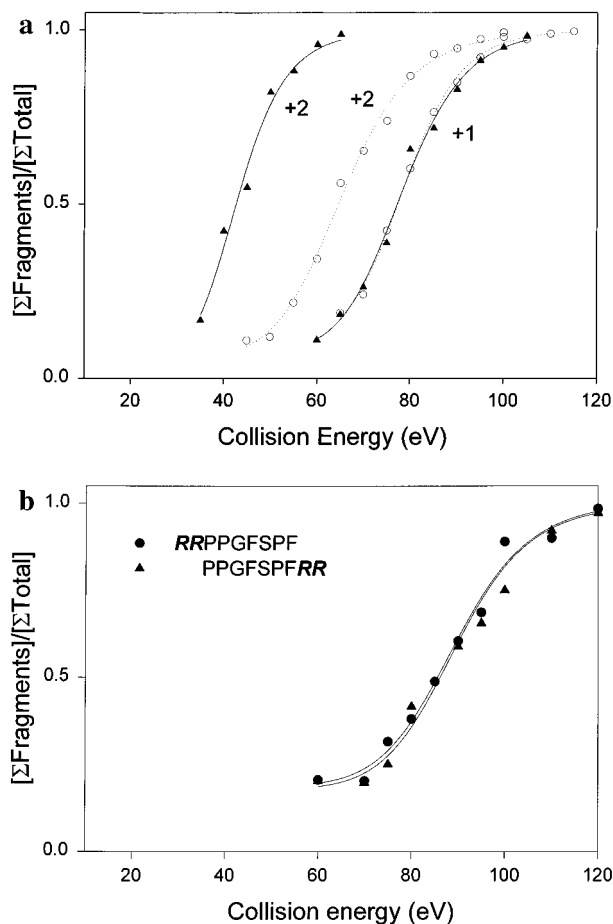
Figure 4. Fragmentation efficiency curves (ESI/SID) for the singly- and doubly-protonated forms of des-Arg 9 bradykinin ( RPPGFSPF ) (represented by ▲/—) and des-Arg 1 bradykinin ( PPGFSPFR ) (represented by ○/---). The y axis represents \Sigma(\text{fragment ion intensity})/\Sigma(\text{total ion intensity}) and the x axis represents SID collision energy. (b) Fragmentation efficiency curves (ESI/SID) for doubly-protonated forms of RRPPGFSPF and PPGFSPFRR . The y axis represents \Sigma(\text{fragment ion intensity})/\Sigma(\text{total ion intensity}) and the x axis represents SID collision energy.
