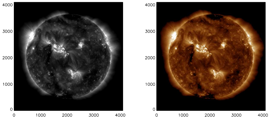
Figure 3: AIA 193 Å data plotted with (left) a greyscale colour table; (right) the proposed AIA 193 Å colour table.
